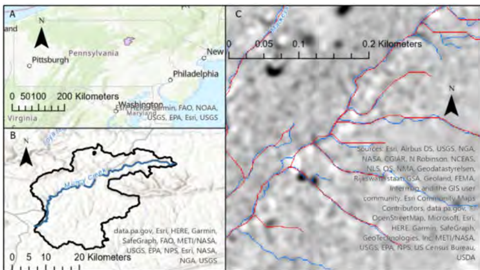
Figure 1. Panel A: location map showing location of Muncy Creek watershed within Pennsylvania, USA (in pink). Panel B: Topographic map showing the watershed area and Muncy Creek. A black dot near the northernmost point in the watershed is the location of panel C. Panel C shows the 2006 flow paths for this site in blue, and the 2017 paths in red. Paths are plotted on top of the E layer, so that pale areas represent erosion and darker areas represent deposition.
